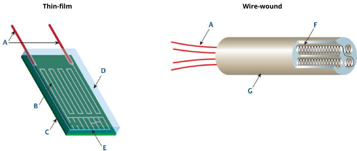
Figure 3: RTD Elements
